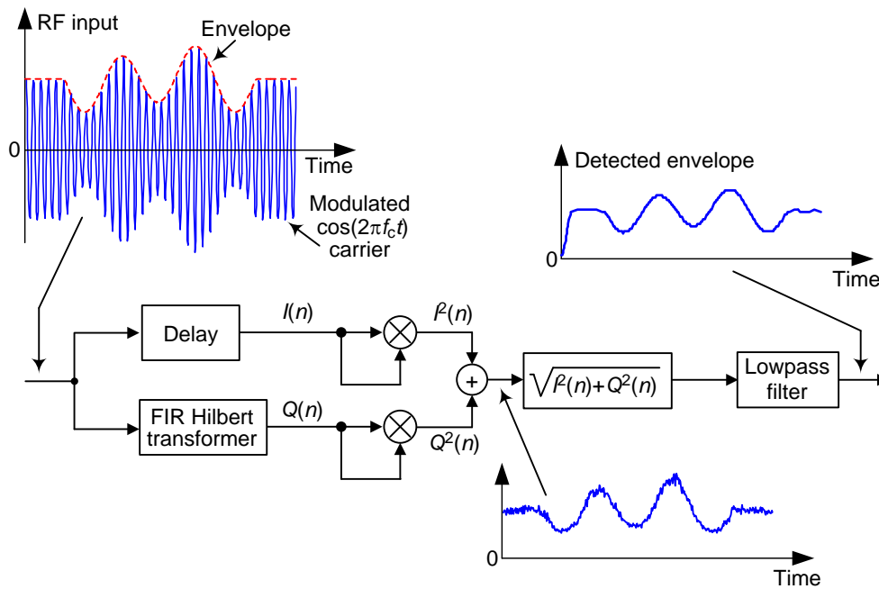
Figure 5: Asynchronous complex square-law envelope detector.
