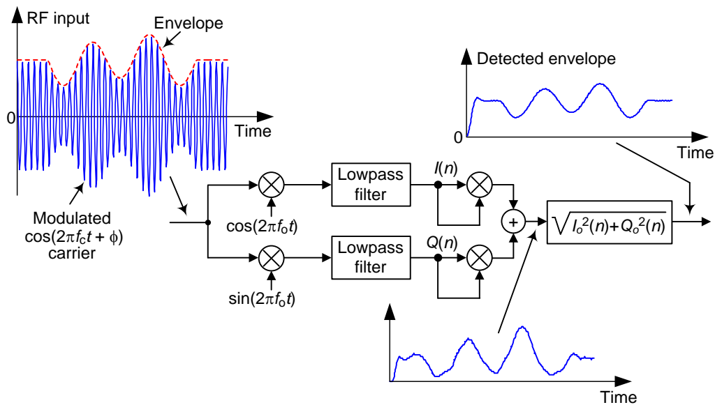
Figure 7: Asynchronous complex envelope detector.
