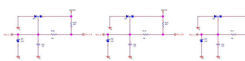
HALL EFFECT CONNECTIONS
