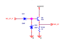
P MOSFET GATE DRIVE
