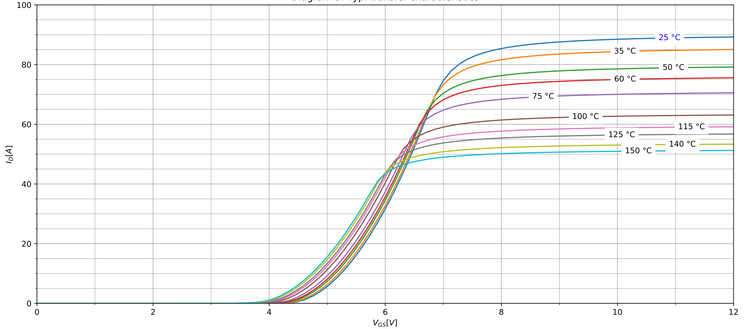
Diagram 9: Typ. transfer characteristics
