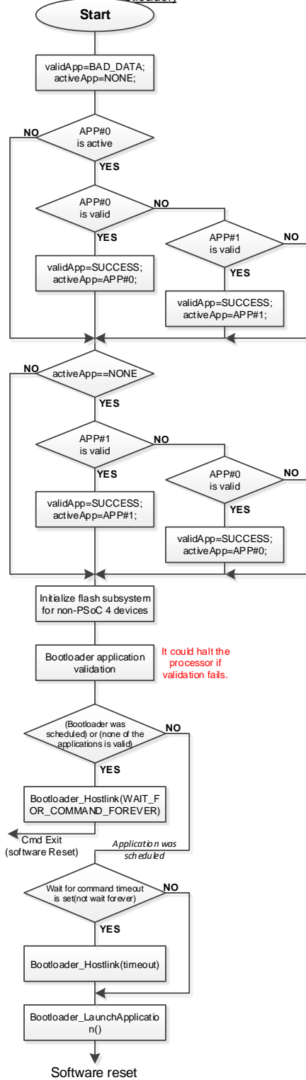
Classic implementation (Dual-application Bootloader)
