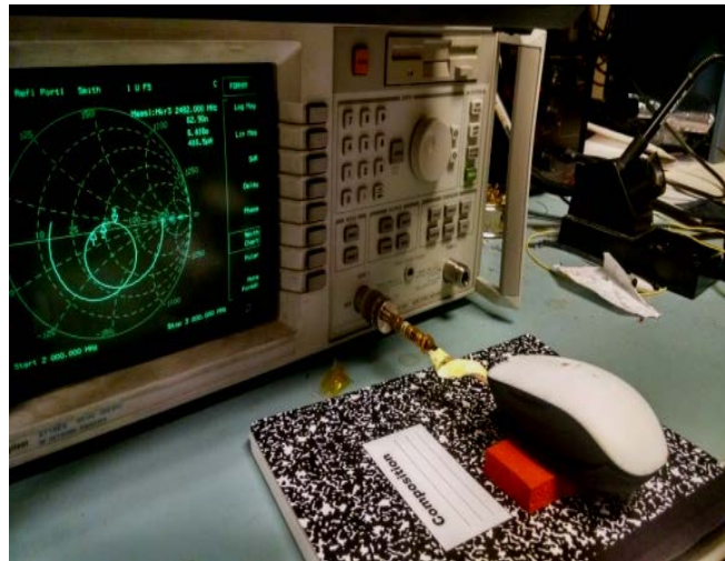
Figure 47. Smith Chart with Plastic Assembly, Illustration of Connecting with ID
