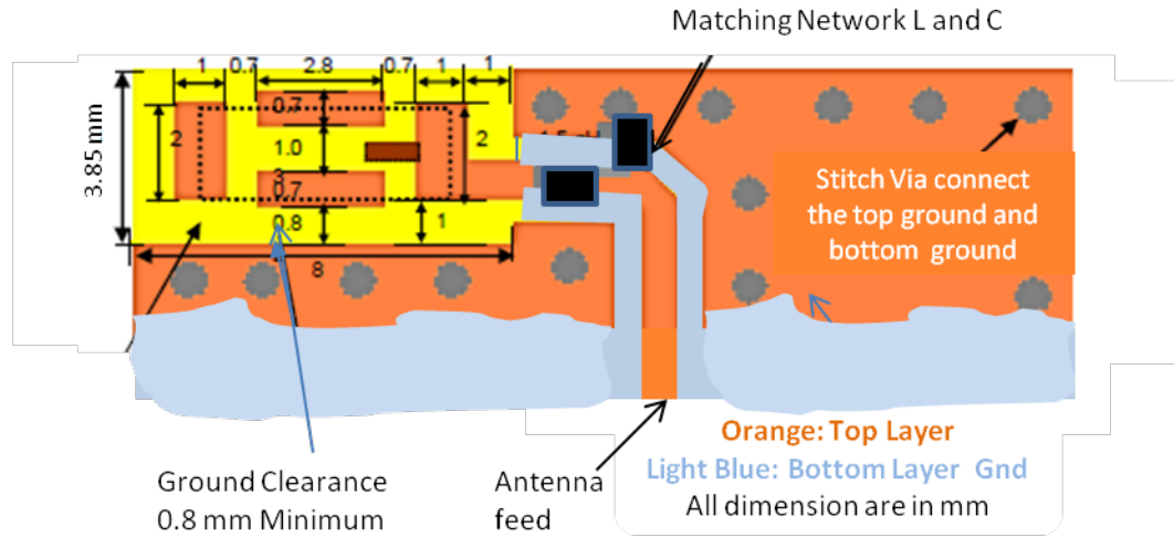
Figure 20. Layout Guideline for Johanson 2450AT42B100E Chip Antenna
